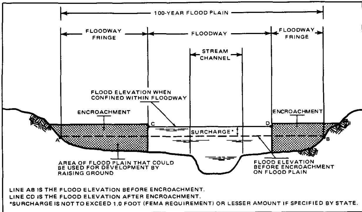
Figure 2. Floodway Schematic
